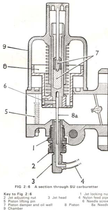
Fig. 2. SU Carburetter cross section.
