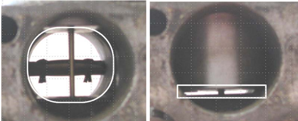
Fig. 1 Full size venturi at wide open throttle (left) and idle condition (right).
