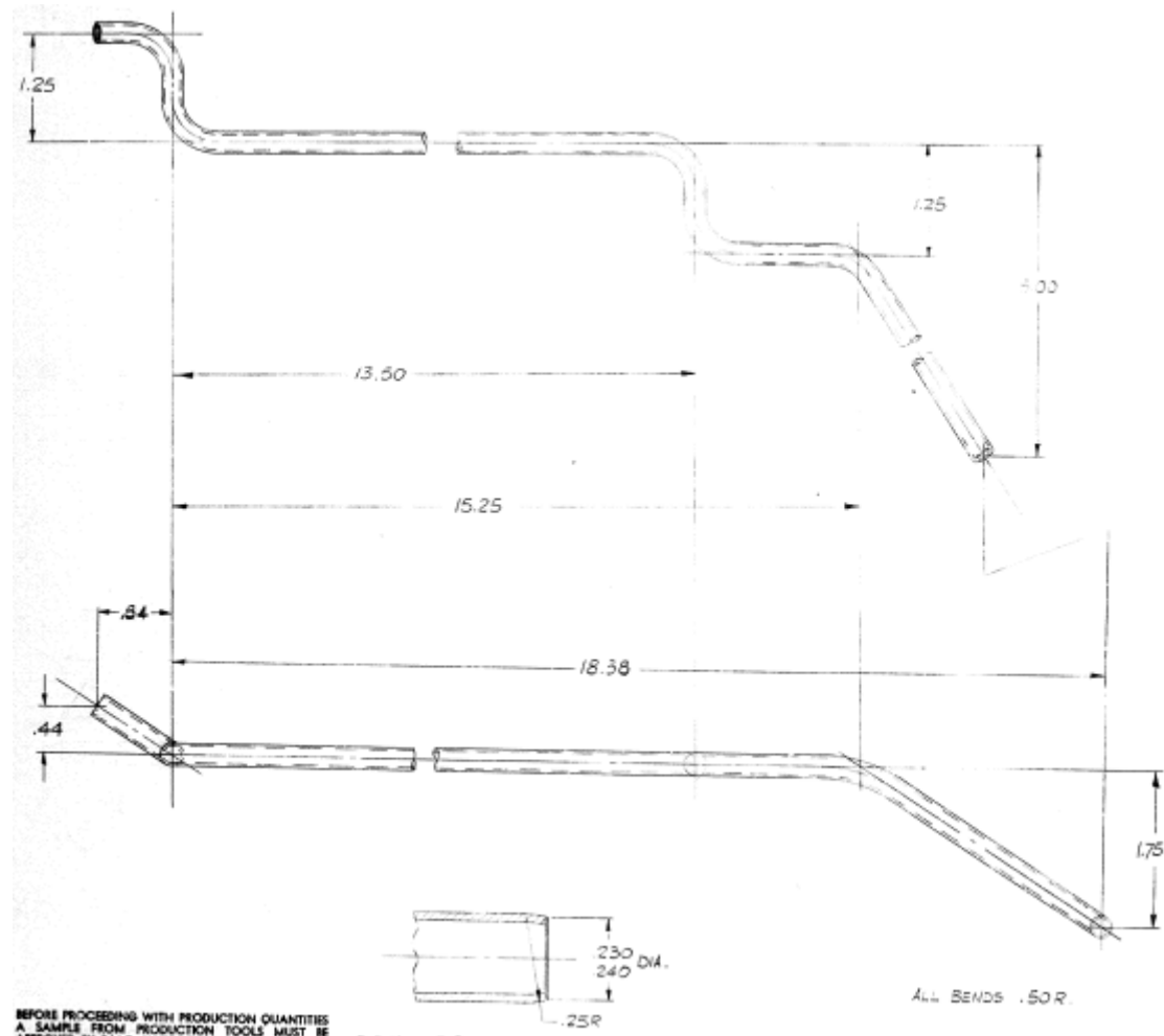
Fig. 5.1.10 Fuel supply pipe AYK2086.
