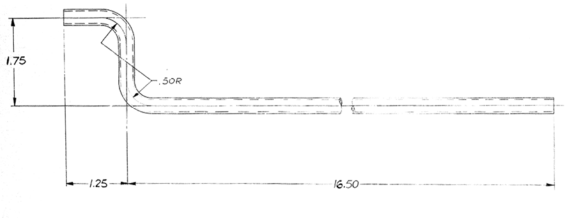
Fig. 5.1.9 Fuel supply pipes AYK2085.
